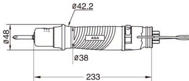
MOT-K50/K55/K60/K65PB
