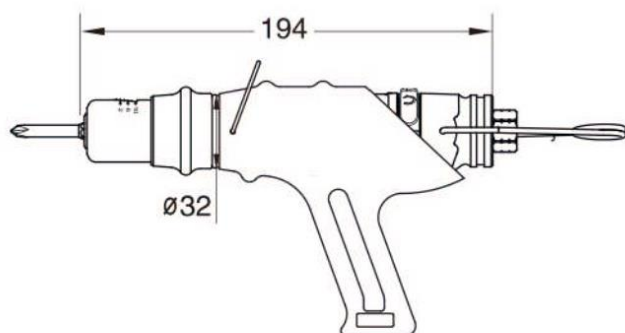
MOT-K10/K20/K30/K40/K45PB/PG
