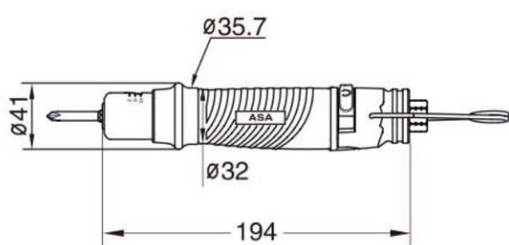
MOT-K10/K20/K30/K40/K45PB
